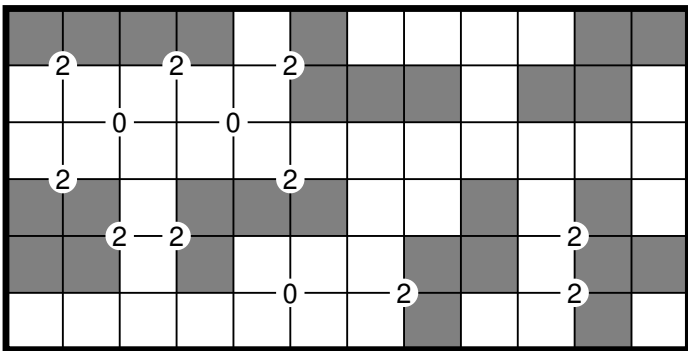
6.3 Tetroscope
