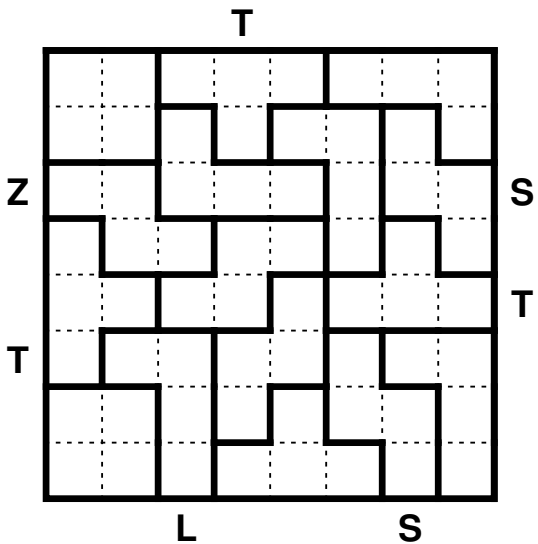
6.4 Tetrominosalat
