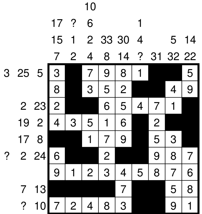
6.7 Tetromino-Yajilin
