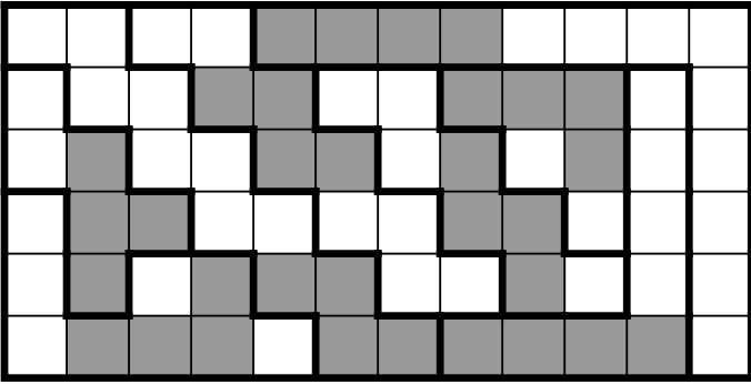
6.1 LITS
