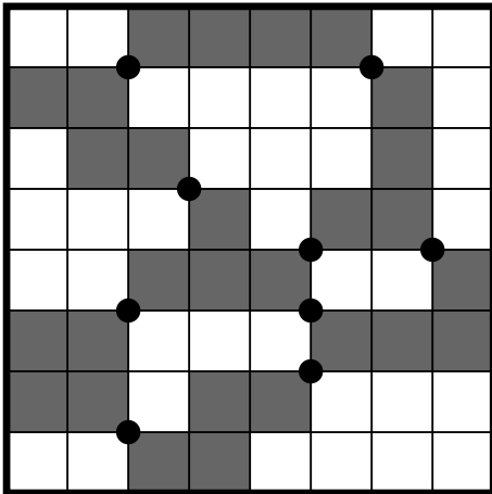
6.2 Touching Tetrominos
