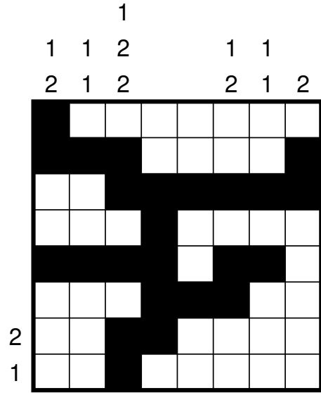
6.5 Tetromino-Koralle
