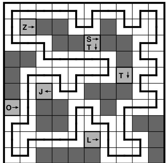
6.7 Tetromino-Yajilin
