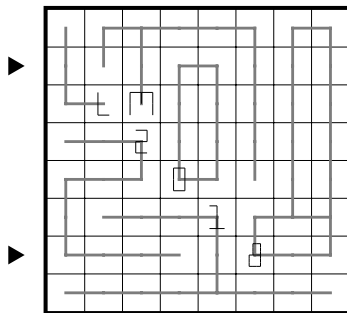
20. Curve Data
